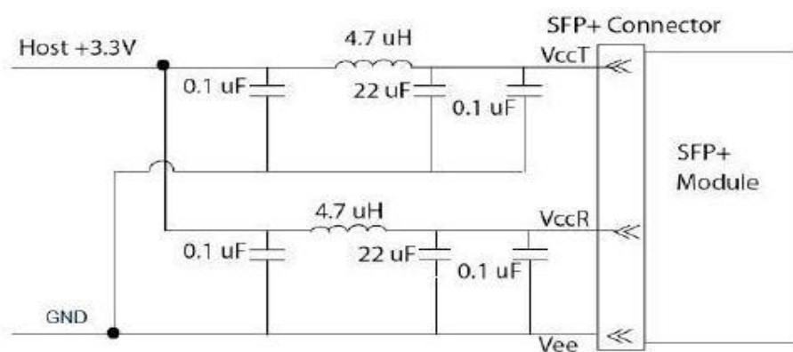
Host Board Power Supply Filters Circuit
