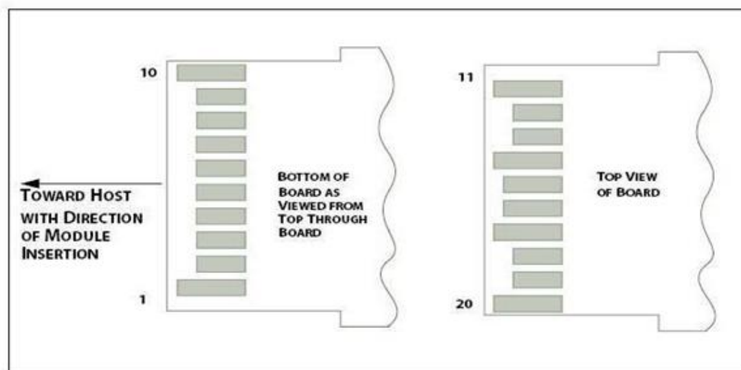
SFP+ module contact assignment
